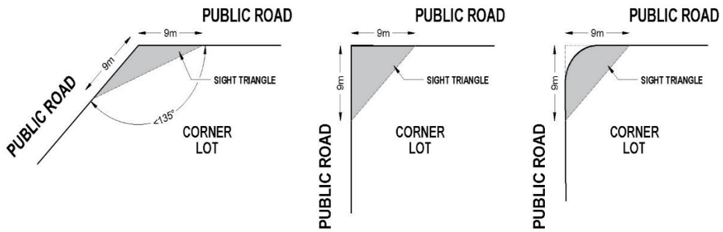
FIGURE 6: YARDS
