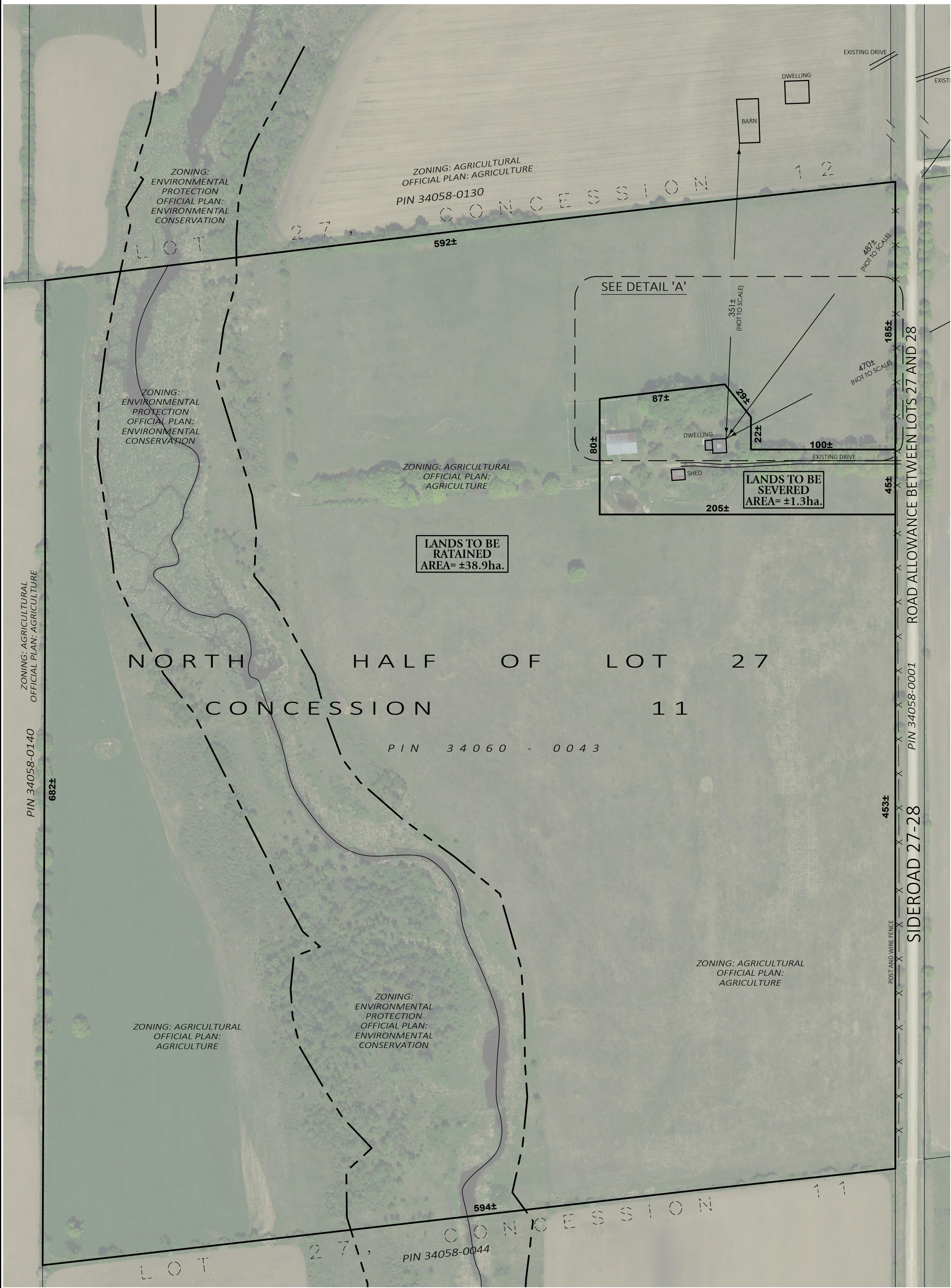
SEVERANCE SKETCH NORTH HALF OF LOT 27, CONCESSION 11 GEOGRAPHIC TOWNSHIP OF EAST LUTHER TOWN OF GRAND VALLEY COUNTY OF DUFFERIN SCALE 1 : 2000 0 20 40 80 120 metres VAN HARTEN SURVEYING INC.
