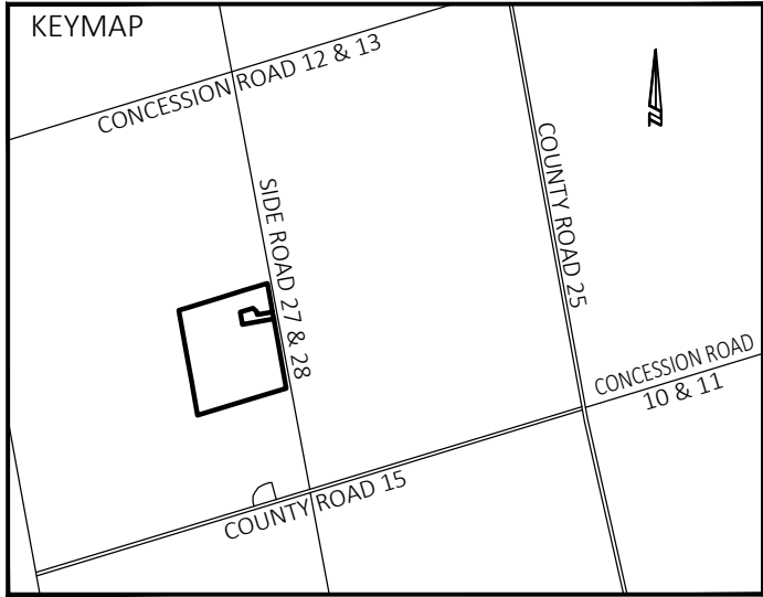
SEVERANCE SKETCH NORTH HALF OF LOT 27, CONCESSION 11 GEOGRAPHIC TOWNSHIP OF EAST LUTHER TOWN OF GRAND VALLEY COUNTY OF DUFFERIN SCALE 1 : 2000 0 20 40 80 120 metres VAN HARTEN SURVEYING INC.
